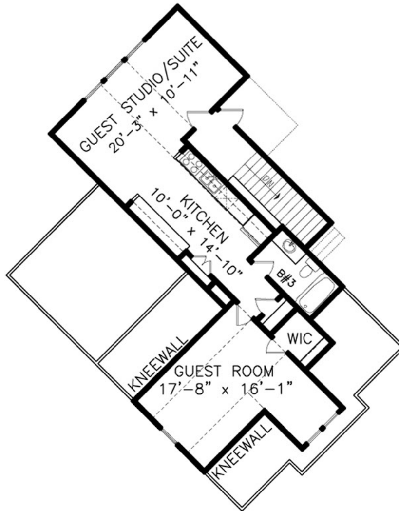
OPT. 2nd FLOOR PLAN 797 SQ. FT.
